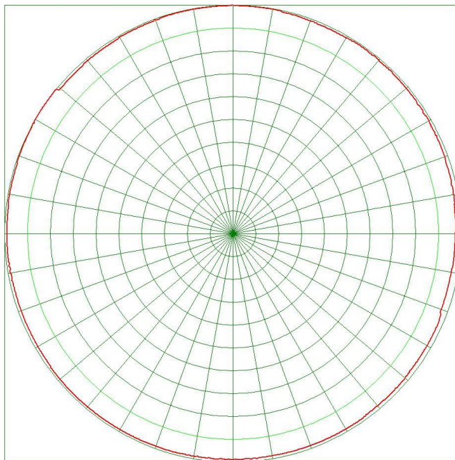
H 面方向图 H plane direction
